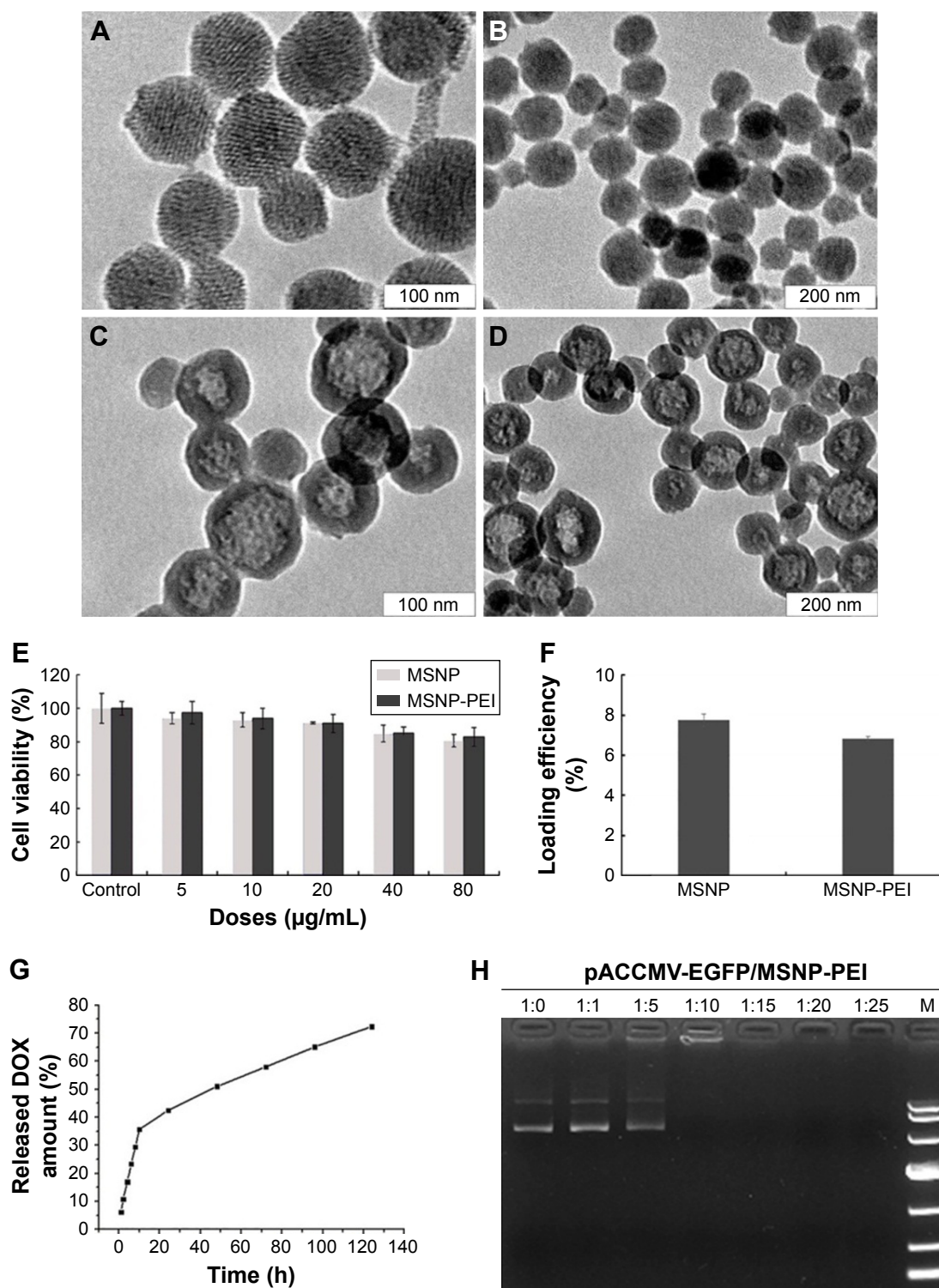
Figure 1 Characteristics of the MSNP and MSNP-PEI nanoparticles.
