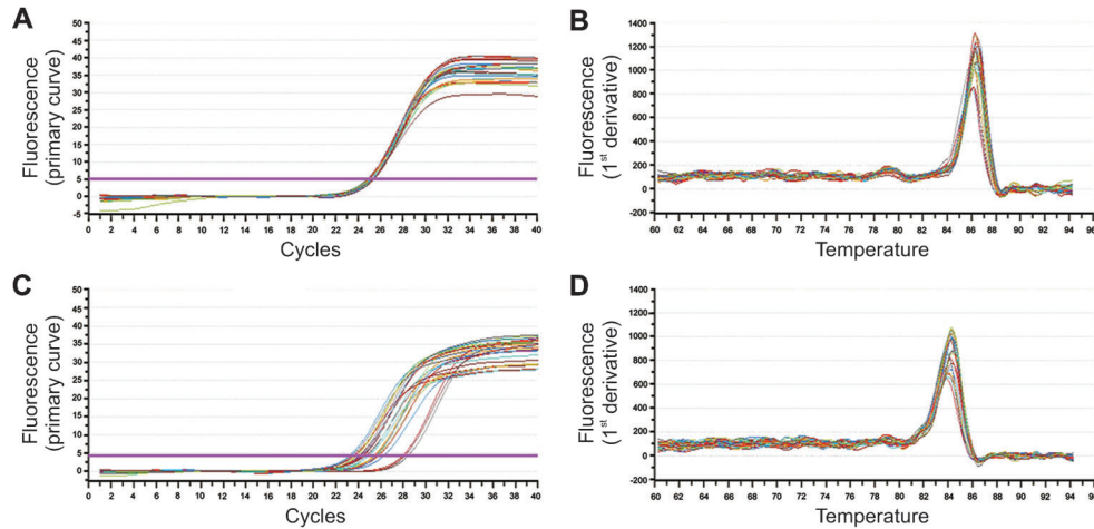
Figure 4. Amplification and dissolution curves for GAPDH and CYP11B2. A, GAPDH amplification curve; B, GAPDH melting curve; C, CYP11B2 amplification curve; D, CYP11B2 melting curve.
