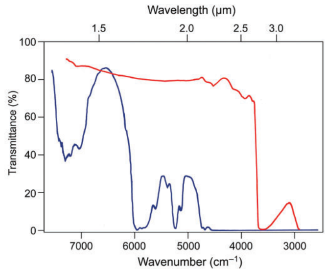
Figure 4. Transmittance spectra of glass (6.5 mm thick; red line) and acrylic (9 mm thick; blue line) plates in the near-infrared region.
