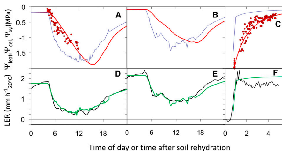
Figure 9. Outputs of the model presented in Figure 8, run with environmental conditions of 2 d with high (A and D; experiment 6) or low (B and E; experiment 9) evaporative demands or in the rehydration experiments (C and F; experiment 2–4). A to C, Red line, leaf water potential ( \Psi_{\text{leaf}} [ \Psi_{\text{cell}} in Fig. 8]); blue line, \Psi_{\text{xyl}} ; red circles, \Psi_{\text{leaf}} measured experimentally. D to F, Green and black lines show simulated and observed LER, respectively.
