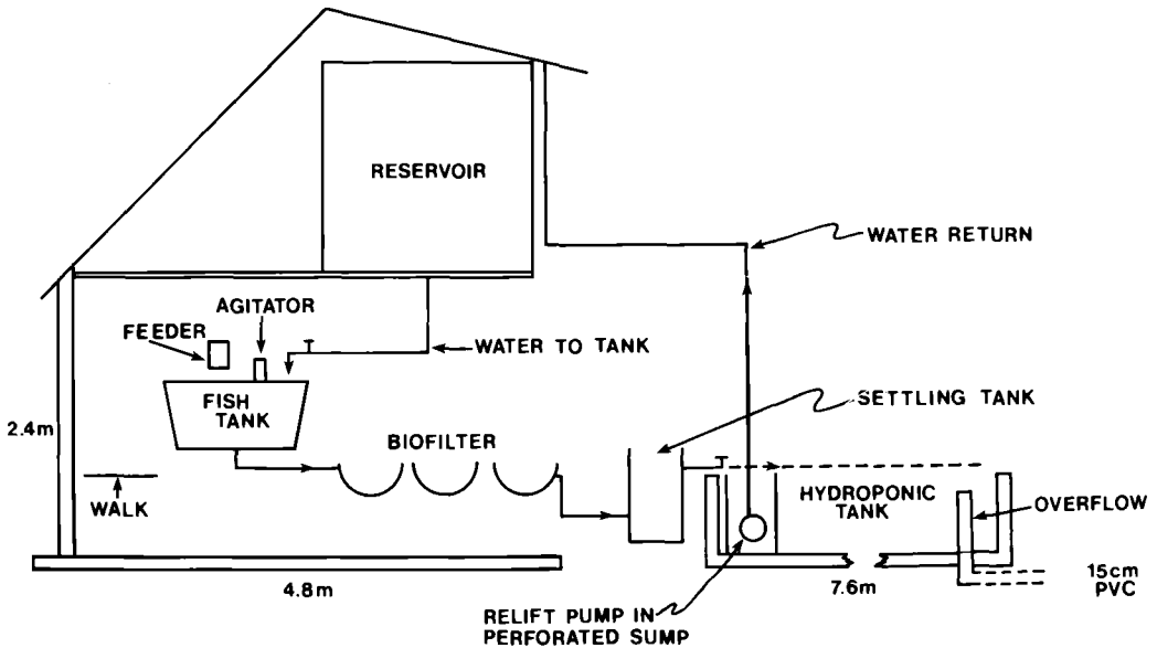
FIGURE 1.—A system combining fish production tanks and hydroponic tanks (elevation).
