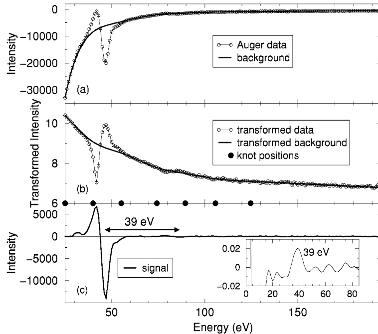
FIGURE 7. (a) An MVV Auger spectrum for iron. The estimated background shown is that obtained for the transformed spectrum shown in (b). (b) A logarithmic transformation of the Auger spectrum shown in (a) reduces the curvature of the background, rendering it suitable for the general approach presented here. The estimated background is shown. (c) The signal determined by subtracting the estimated background from the original spectrum. The inset in (c) shows the autocorrelation of the signal vs. energy difference. A significant secondary peak is seen at an energy offset of 39 eV.
