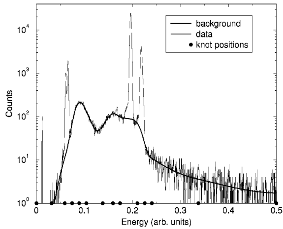
FIGURE 4. The same PIXE spectrum as in Fig. 1, showing the most probable background estimate obtained using adaptive splines in which the optimal number of knots is found to be 14. In the energy region above 0.25, the estimated background is now smooth, indicating a lack of evidence in the data for the oscillations visible in Fig. 1.
