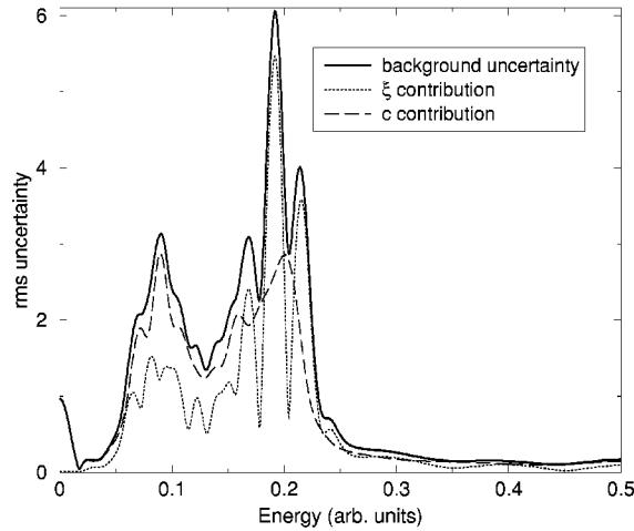
FIGURE 6. The uncertainties in the background function displayed in Fig. 4. The separate contributions to the rms deviation of the background values are shown; from the uncertainties in the c and the variance arising from the knot positions \xi .
