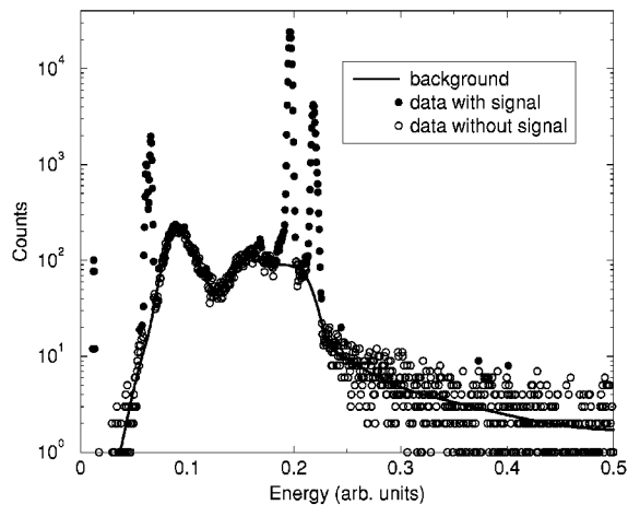
FIGURE 5. Data points classified with a background probability greater than 50% as background-only points are depicted by open circles while data points carrying a signal contribution are marked by solid circles.
