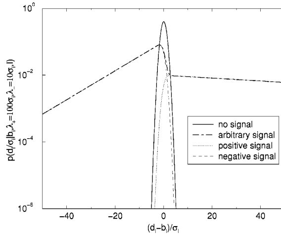
FIGURE 2. The likelihood functions for the cases that there is no signal present, and for positive and negative signals of scales \lambda_- = 10\sigma and \lambda_+ = 100\sigma . The relative contribution of the latter to the mixture model (12) for the likelihood is weighted by 1 - \beta , and the former by \beta .
