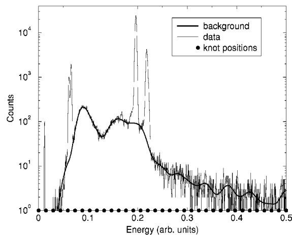
FIGURE 1. A PIXE spectrum for a geological sample with the background estimate obtained in Ref. 1 using 35 evenly spaced spline knots. The oscillations in the estimated background above the energy of 0.25 seem unwarranted, given the large uncertainties in the measurements in this region.
