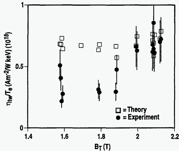
FIGURE 9. Toroidal magnetic field dependence of the FWCD efficiency normalized to the central electron temperature.
