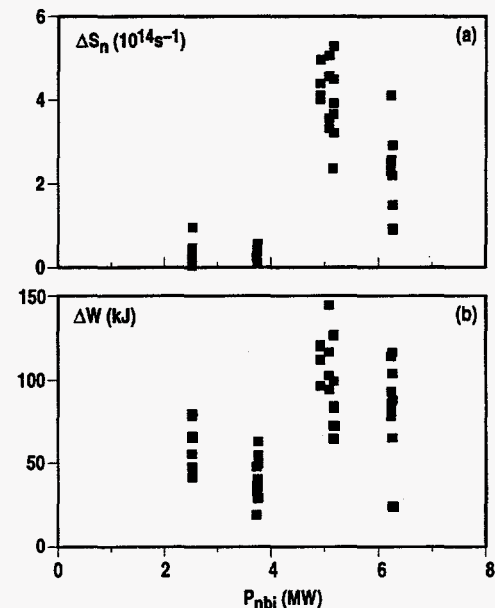
FIGURE 8. Dependence of the (a) anomalous neutron rate and (b) anomalous fast ion stored energy on the neutral beam power ( B_T = 2.1 T, \bar{n} = 2.1 \times 10^{19} \text{ m}^{-3} , P_{fw} \approx 2.2 MW).
