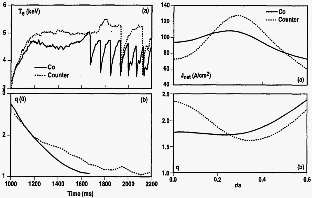
FIGURE 5. Radial profiles of (a) net current density and (b) safety factor at identical times for matched co and counter FWCD discharges ( B_T = 1.9 T, \bar{n} = 1.3 \times 10^{19} \text{ m}^{-3} , \bar{n} = 1.8 \times 10^{19} \text{ m}^{-3} , P_{nbi} = 3.7 MW, P_{fw} = 2.2 MW).
