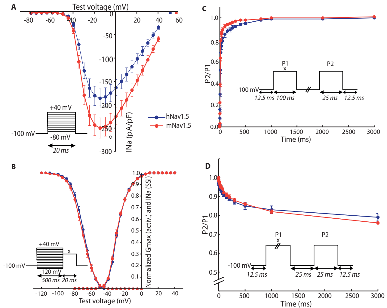
Figure 2. Electrophysiological properties of human and mouse \text{Na}_v1.5 . The voltage-clamp protocols used are shown in the corresponding insets. For B–D , the voltage x was adjusted to the voltage that elicited maximum current during the current voltage ( I/V )-protocol ( -10 to -30 mV). (A) I/V -protocol for assessment of reversal potentials. Peak currents were measured for both channels at -15 mV. Calculated reversal potentials are marked with square data points. (B) Voltage-dependence of activation and steady-state inactivation (SSI). The data was fitted with the Boltzmann formula. Only the slope of the inactivation curve differs between mouse and human sodium channels (shallower in \text{mNa}_v1.5 ). (C) Recovery from inactivation. The duration between the depolarising steps was varied from 0.25 to 3000 ms. \text{mNa}_v1.5 had a slight tendency to recover faster than \text{hNa}_v1.5 . (D) Onset of slow inactivation. The duration of the first step was varied from 0.25 to 3000 ms. The relative number of channels entering slow inactivation is similar for both types. (A–B) n(\text{hNa}_v1.5) = 22 , n(\text{mNa}_v1.5) = 17 . (C–D) n(\text{hNa}_v1.5) = 9 , n(\text{mNa}_v1.5) = 7 . ** P < 0.01 obtained by two-tailed Student's t -tests; error bars indicate standard errors.
