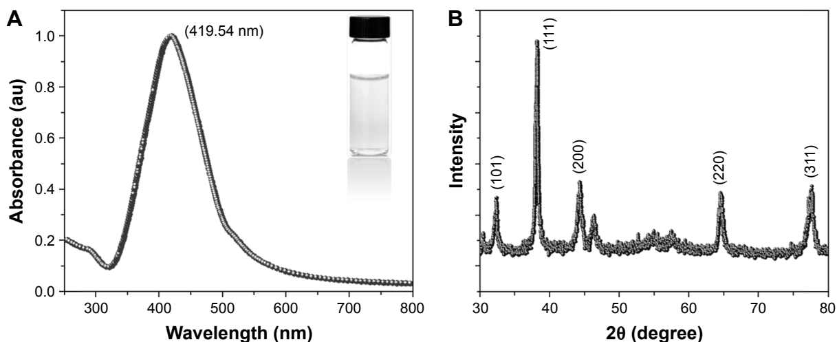
Figure 1 (A) UV-visible spectra of AgNPs, (B) XRD pattern of AgNPs. Abbreviations: AgNPs, silver nanoparticles; UV, ultraviolet; XRD, X-ray diffraction.
