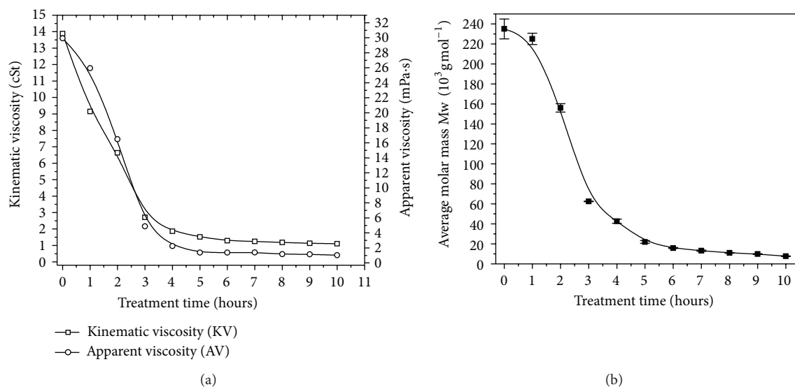
FIGURE 1: Kinematic and apparent viscosities (a) and average molar mass (b) of chitosans in solid state thermally degraded at 100^\circ\text{C} for up to 10 h.
