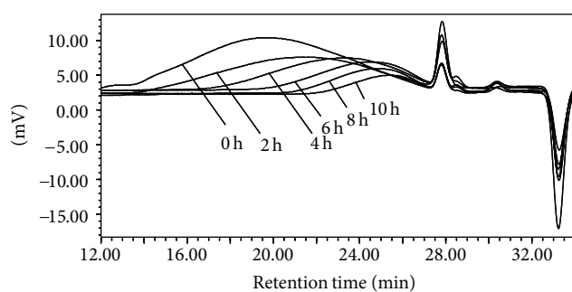
FIGURE 2: Chromatographic profiles obtained by GPC for control chitosan without thermal treatment (0 hour) and chitosans treated for up to 10 h.
