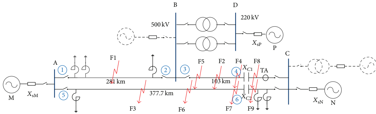
FIGURE 1: Simulation model of power grid.
