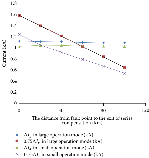
FIGURE 2: The relationships of \Delta I_d and 0.75\Delta I_r , when the single phase grounding fault with 300\ \Omega transition resistance occurred at different places on the line BC.
