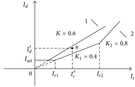
FIGURE 3: The characteristic curves of segregated phase current differential protection.
