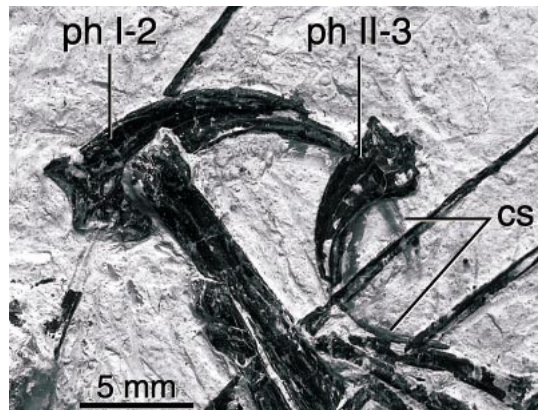
Fig. 22. Manual unguals of CAGS 20-8-001.
