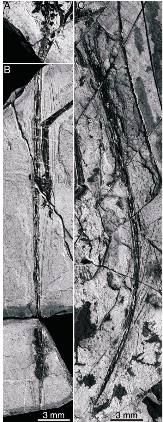
Fig. 10. Tails of the Microraptor specimens. (A) Anterior caudal vertebrae of CAGS 20-8-001 on slab. (B) Remainder of caudal vertebrae of CAGS 20-8-001 on counterslab. (C) Caudal vertebrae of CAGS 20-7-004. Note the rodlike extensions of the prezygapophyses and chevrons that surround and stiffen both tails.
