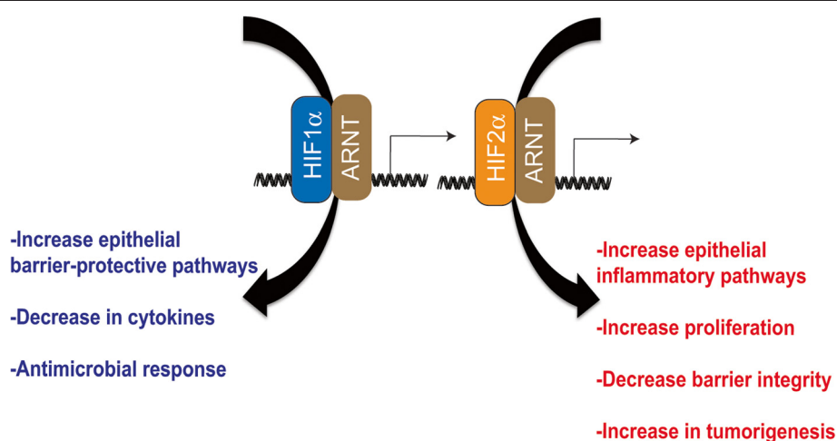
Fig. 2 Distinct roles of HIF-1 \alpha and HIF-2 \alpha in IBD. Activation of HIF-1 \alpha increases barrier protective genes and activates a protective innate immune response and antimicrobial response. HIF-2 \alpha activation in the intestine leads to an increase in pro-inflammatory mediators and decrease barrier integrity and results in increase susceptibility to colon tumors. ARNT aryl hydrocarbon receptor nuclear translocator, HIF hypoxia-inducible factor
