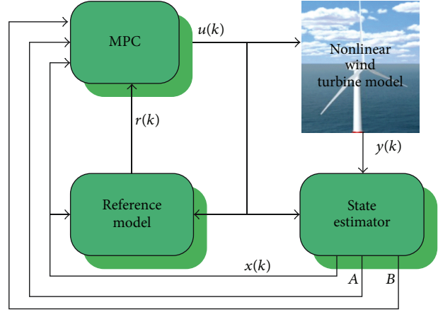
FIGURE 2: Wave disturbance using MPC.
