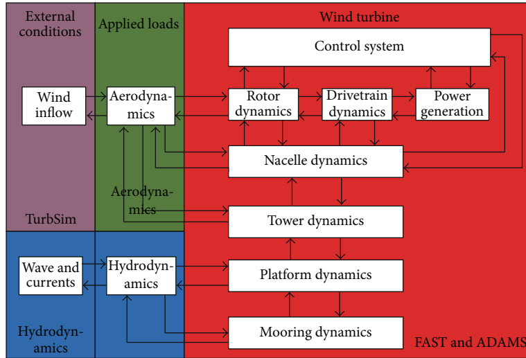
FIGURE 4: Offshore FAST structure (from NREL).
