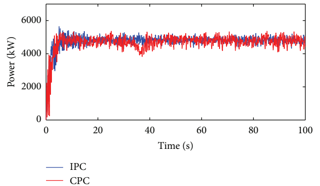
FIGURE 7: Power output.
