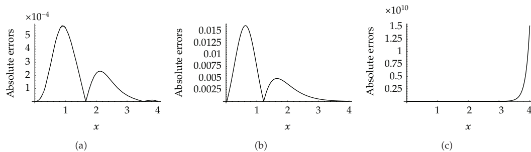
Figure 2: Comparison of absolute errors using the present method, MVIM [9] and VIM [6] for Example 4.1. ((a): The present method; (b): MVIM [9]; (c): VIM [6]).
