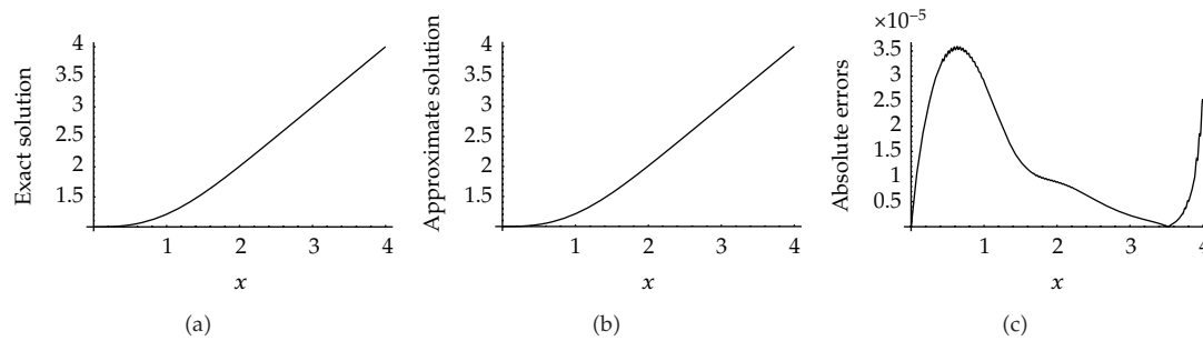
Figure 3: The numerical results for Example 4.3. ((a): exact solution; (b): approximate solution; (c): absolute error.).
