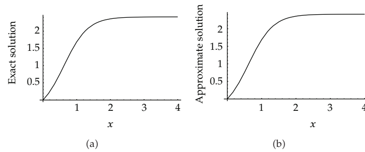
Figure 1: Comparison of approximate solutions with the exact solutions for Example 4.1. ((a): exact solution; (b): approximate solution.).
