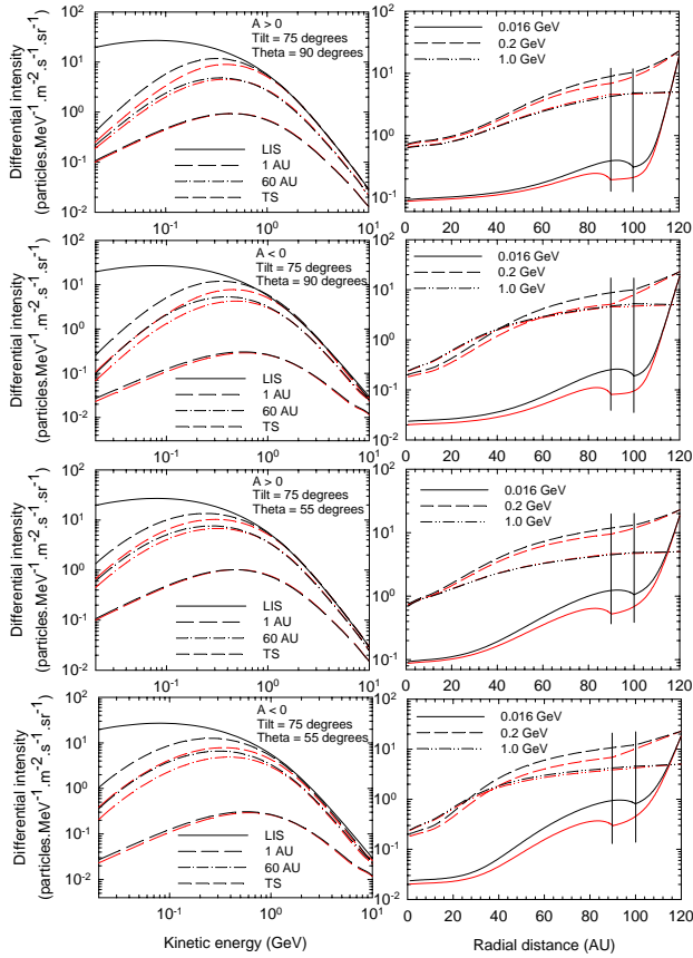
Fig. 2. Similar to Fig. 1 but with the TS positioned at 90 AU (red curves) and 100 AU (black curves), respectively, as indicated with the heliopause position specified at 120 AU.
