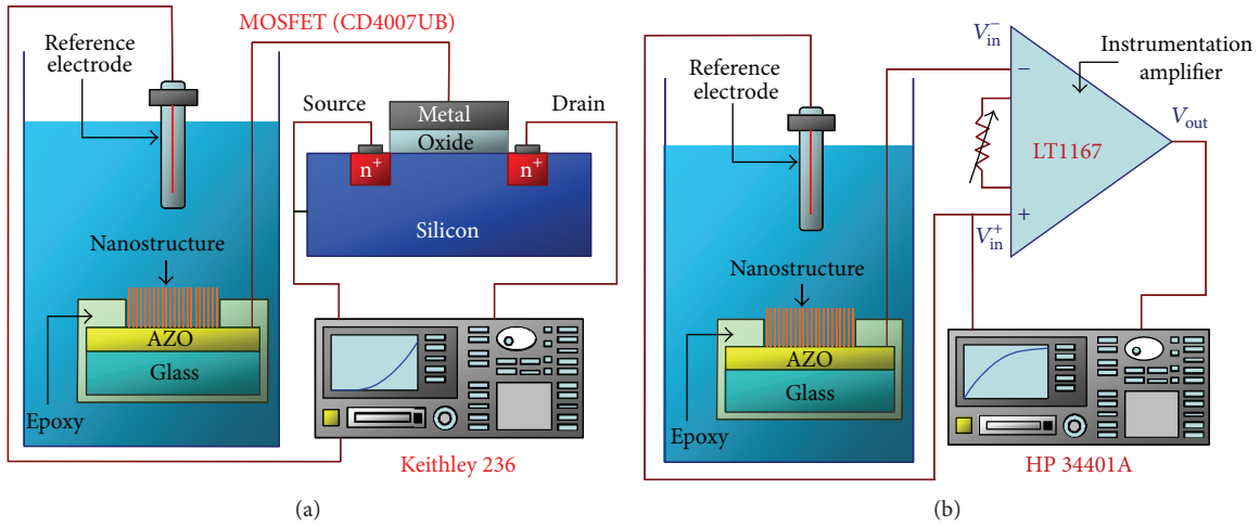
FIGURE 2: Schematic diagrams of the (a) I - V measurement facility and (b) V - t measurement system for the pH-EGFET sensors.
