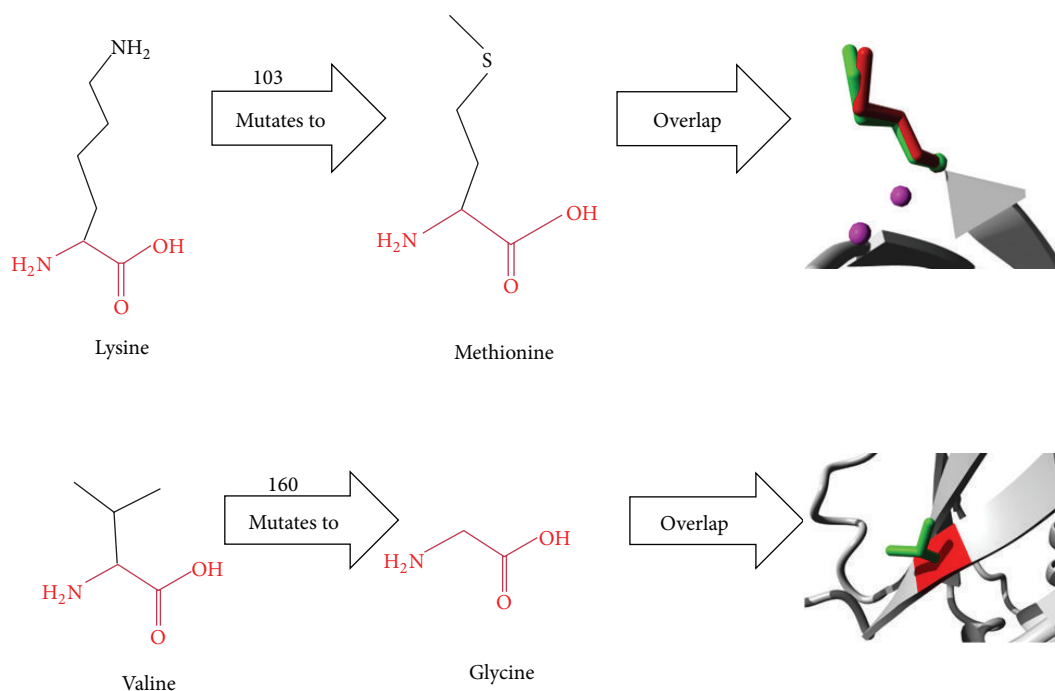
FIGURE 1: Schematic structure of the wild type and mutant (Lys103Met and Val160Gly) amino acids.
