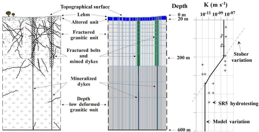
Figure 7. Schematic vertical section representing variations in data derived from the hydraulic characterization of borehole SR5 (500 m deep) indicate that hydraulic conductivity changes with depth. This fact was studied by Stober (1997). The model uses a modification of Stober’s equation: hydraulic conductivity is kept constant up to the base of the fractured granitic unit (200 m), then changes with depth down to 350 m. From there, it remains constant down to the model bottom.
