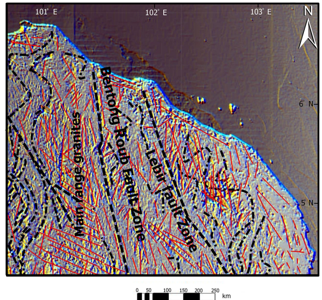
Figure 6. ScanSAR image map derived from N-S (0°), NE-SW (45°) and NW-SE (135°) directional filters for the northern part of the Peninsular Malaysia. The explanation for the figure: dashed black lines are major faults; dot-dashed lines are folds and curvilinear; red lines are faults and fractures.
