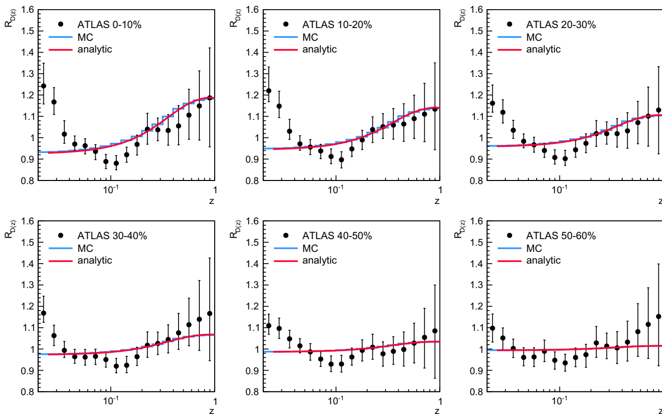
Fig. 9 Ratios of D(z) distributions for six bins in collision centrality to those in peripheral (60–80 %) collisions, D(z)|_{\text{cent}}/D(z)|_{60-80} , measured by ATLAS for R = 0.4 jets [12] (black markers) are compared to
