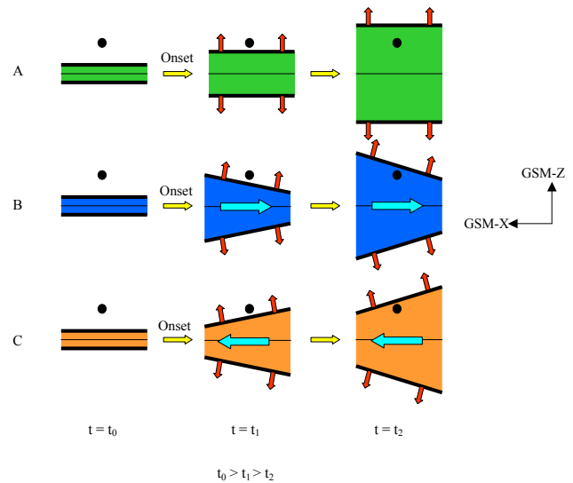
Fig. 20. The normal vectors (red) of the lobe – plasma sheet boundary as the plasma sheet expands: (A) uniformly down the X axis; (B) tailwards from near the Earth; (C) and, earthwards from tailward of the spacecraft. For each case, the plasma sheet prior to onset and its subsequent expansion is shown. Any propagation direction of the expansion is also shown (cyan). The spacecraft quartet is shown as a black circle.
