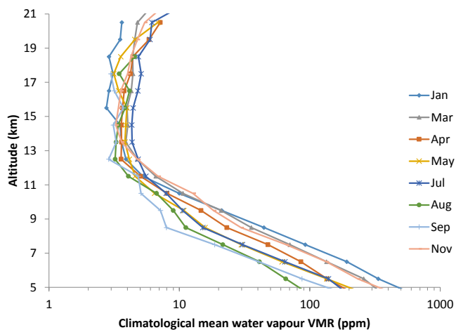
Figure 4. MAESTRO mean climatology (2004–2012) of the vertical distribution of the water vapour volume mixing ratio in the Antarctic (60–90° S) UTLS for months with sufficient sampling of the region. A logarithmic scale is used for the x axis.
