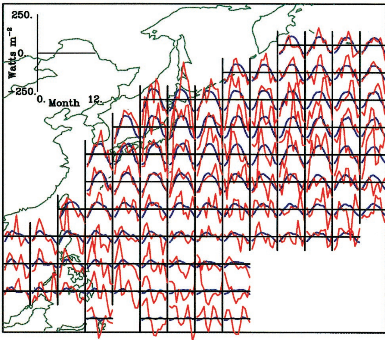
FIG. 9. Climatologies of the demeaned net heat flux (blue) and heat storage rates (red) obtained by integrating the temperature profiles down to (a) 300 m, (b) the isotherm whose temperature is one degree less than the coldest observed SST for that grid region. The individual plots are drawn over the 5^\circ \times 5^\circ grid region from where the temperature data was obtained. All temperature profiles within the outlined blue box (b) were normalized to the local 300-m mean temperature. The region outlined by the blue box (b) is also the region compared in Fig. 10. The black boxes indicate the grid location of OWS Papa and November, whose time series were shown in Figs. 7 and 8, respectively.
