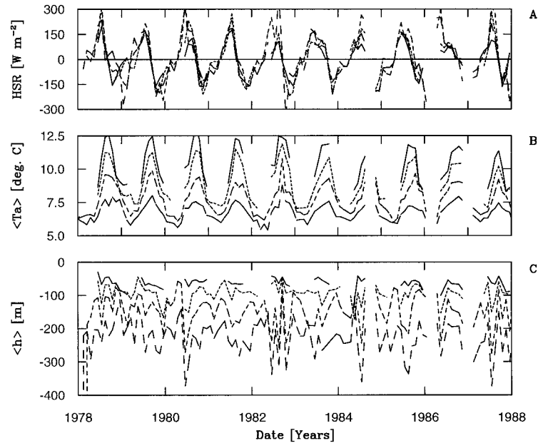
FIG. 2. Sensitivity of (a) \rho c_p \langle h \rangle \langle \partial T_a / \partial t \rangle , (b) \langle T_a \rangle , and (c) \langle h \rangle to changes in the choice of isotherm ( 3^\circ – 6^\circ\text{C} , by 1^\circ increments) down to which the temperature profile (XBT/CTD) data were integrated. The time series presented here used data obtained from the 45^\circ – 50^\circ\text{N} , 145^\circ – 140^\circ\text{W} region.
