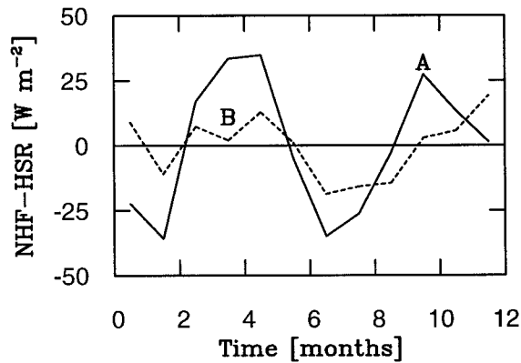
FIG. 10. Regional ( 20^{\circ} – 55^{\circ} N, 180^{\circ} – 115^{\circ} W) mean difference between the demeaned net heat flux and heat storage rate climatologies obtained by integrating the temperature profiles down to (a) (solid line) the isotherm whose temperature is 1^{\circ} C colder than the coldest observed SST for that specific 5^{\circ} \times 5^{\circ} grid region and (b) (dashed line) the same isotherm as in (a) but after normalizing each temperature profile to the local 300-m mean temperature.
