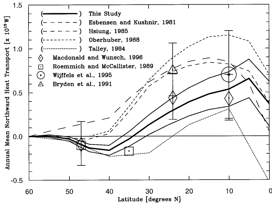
FIG. 13. The annual mean northward heat transport (petawatts) for the North Pacific obtained by integrating the annual mean net heat flux estimates using data from this study (thick solid line), and the previous studies of Talley (1984), Oberhuber (1988), Hsiung (1985), and Esbensen and Kushnir (1981). The error estimate from this study obtained from an estimated \pm 20 \text{ W m}^{-2} rms error and a 7% bias on the annual mean is shown with the thin solid line. The latitude-specific estimates of northward heat transport from Macdonald and Wunsch (1996), Roemmich and McCallister (1989), Bryden et al. (1991), and Wijffels (1995) are also shown.
