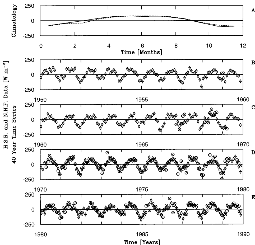
FIG. 8. As in Fig. 7 but to OWS November.
