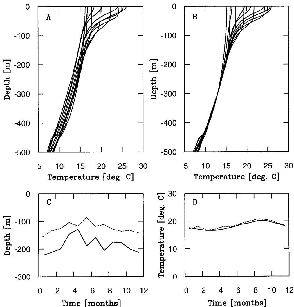
FIG. 3. The mean monthly temperature profiles from the 35^{\circ} – 40^{\circ} N, 165^{\circ} – 170^{\circ} E bin (a) before and (b) after normalization of each profile to the mean 300-m temperature. The time series of (c) \langle h \rangle and (d) \langle T_a \rangle for before (solid) and after (hatched) normalization are shown.
