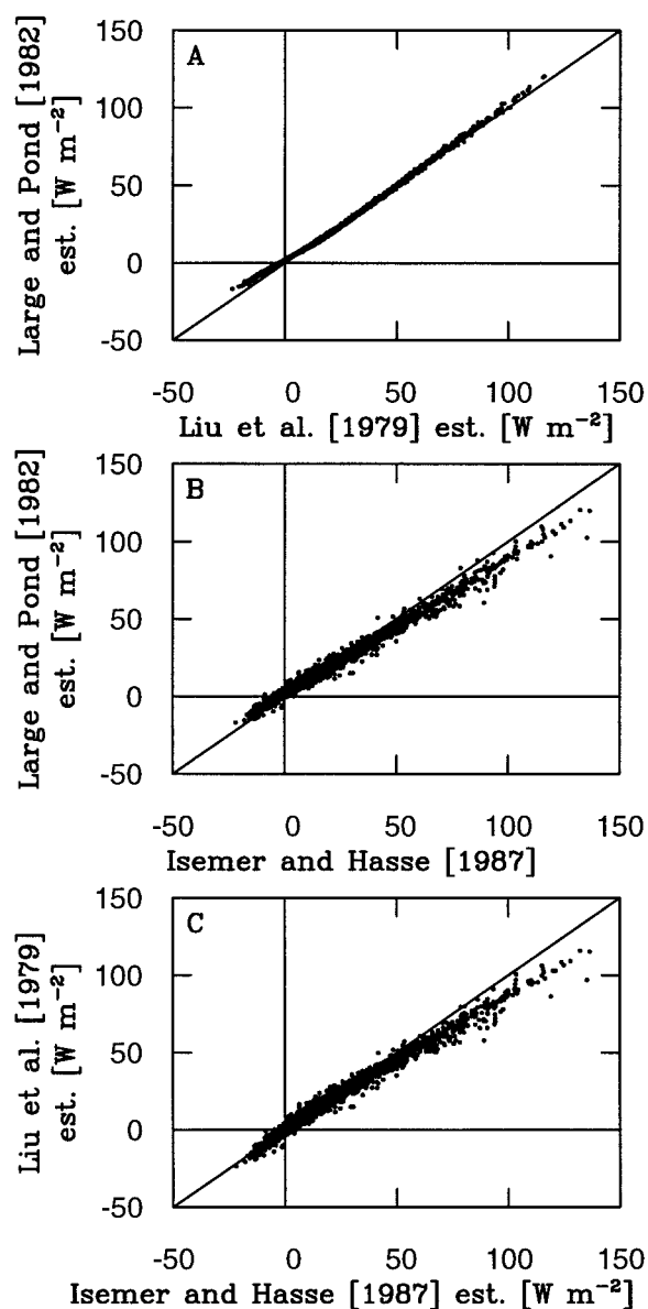
FIG. 6. An intercomparison of the climatological sensible heat flux estimates obtained from the bulk formulas of Large and Pond (1982), Liu et al. (1979), and Isemer and Hasse (1987).
