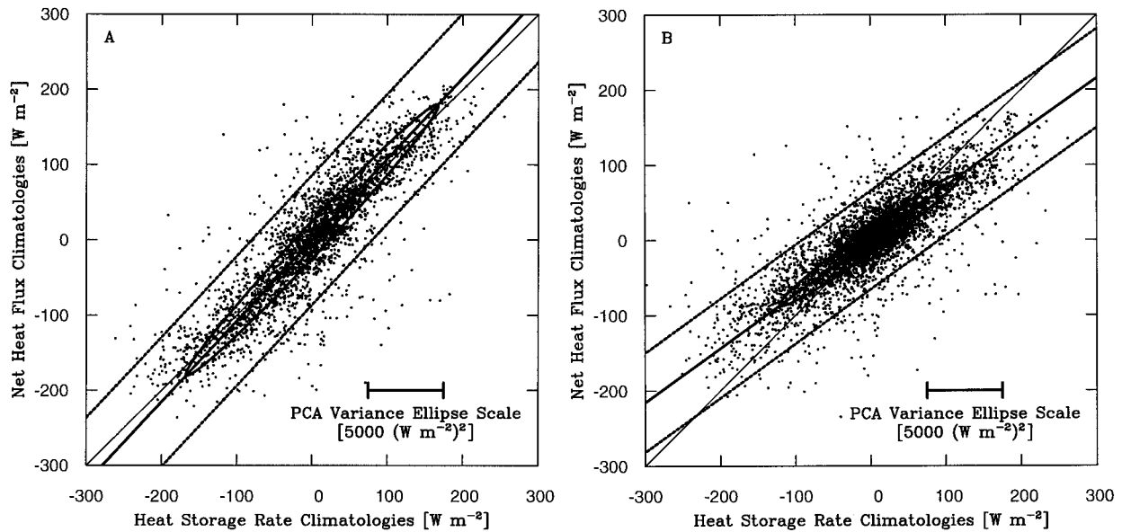
FIG. 14. A comparison of the demeaned net heat flux and net heat storage rate climatologies obtained using the latent and sensible heat flux estimates of (a) Liu et al. (1979) and (b) Large and Pond (1988), and the cloud correction from (a) this study and (b) Reed (1977). The angle of the principal component and the variance ellipse (thick curve and solid line) is used to define the amount of bias and error, respectively, between the estimates. The scale of the variance ellipse is shown in the bottom right of the plot. The dashed lines bracket the region encompassing twice the standard deviation of the values about the principal axis.
