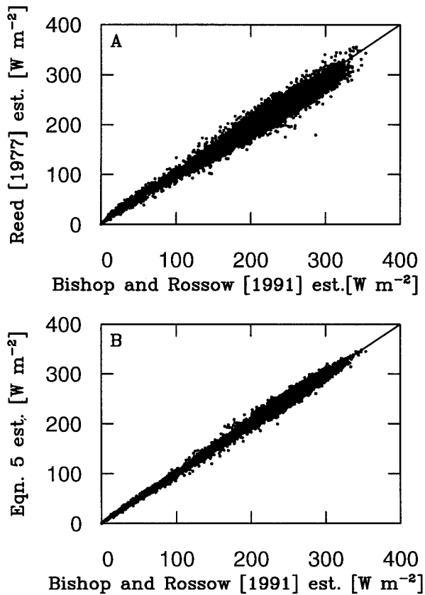
FIG. 4. Comparison of the climatological values for the solar shortwave irradiance flux at the ocean surface between the Bishop and Rossow (1991) dataset and the Bird (1984) solar irradiance model with COADS cloud data and the (a) Reed (1977) and (b) nonlinear [Eq. (5)] cloud correction.
