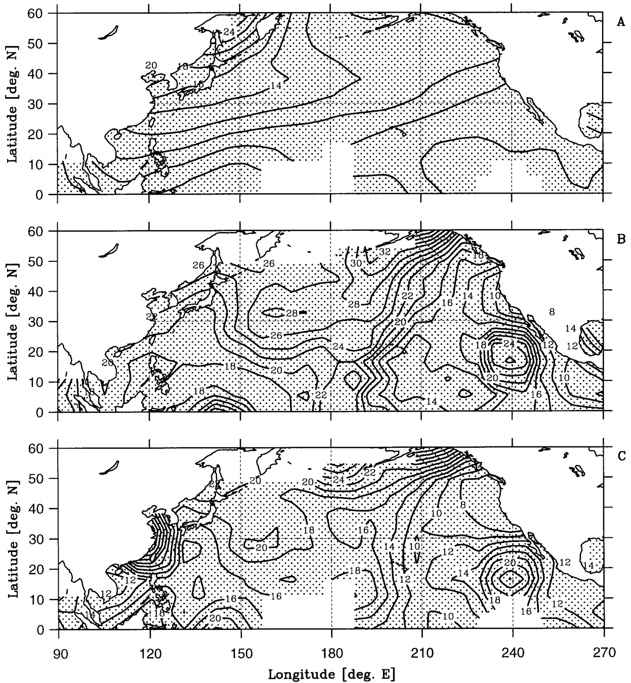
FIG. 12. Uncertainty estimate for the (a) net heat flux climatology, (b) heat storage rate climatology, and (c) the difference between the demeaned net heat flux and heat storage rate climatologies.
