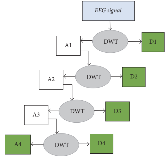
FIGURE 4: EEG signal decomposition through 4-level DWT.
