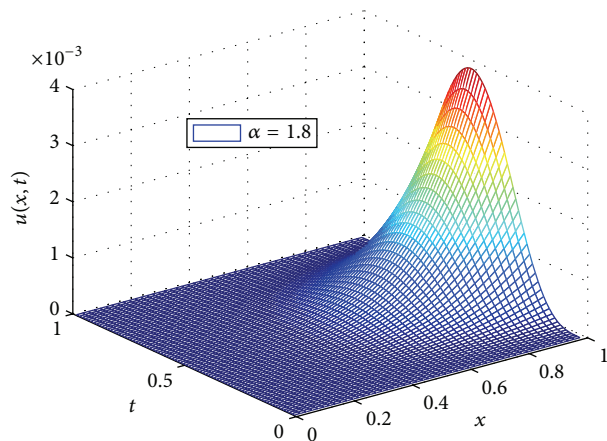
FIGURE 6: The analytical solution surface when \alpha = 1.8 in Example 3.
