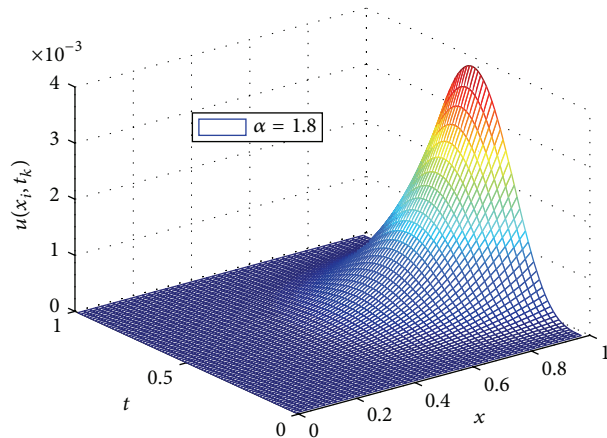
FIGURE 5: The numerical solution surface when \alpha = 1.8 in Example 3 ( \tau = 1/50, h = 1/80 ).
