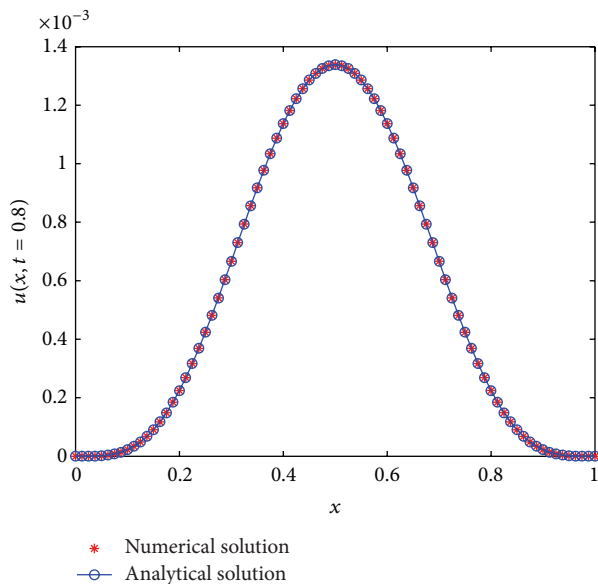
FIGURE 2: Comparison between the analytical solution and the numerical solution at t = 0.8 with \alpha = 1.9 in Example 3 ( \tau = 1/100, h = 1/80 ).
