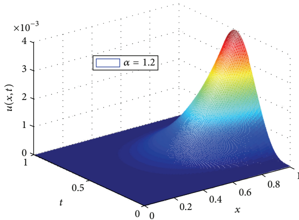
FIGURE 4: The analytical solution surface when \alpha = 1.2 in Example 3.
