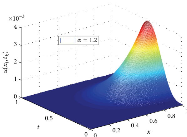
FIGURE 3: The numerical solution surface when \alpha = 1.2 in Example 3 ( \tau = 1/500, h = 1/100 ).
