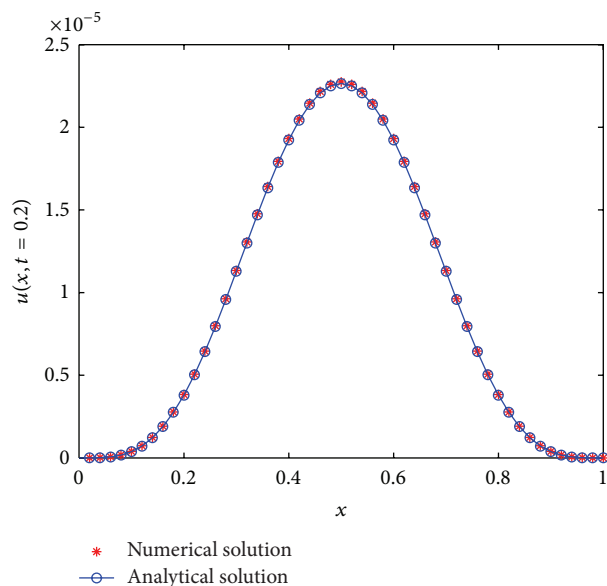
FIGURE 1: Comparison between the analytical solution and the numerical solution at t = 0.2 with \alpha = 1.1 in Example 3 ( \tau = 1/50, h = 1/50 ).
