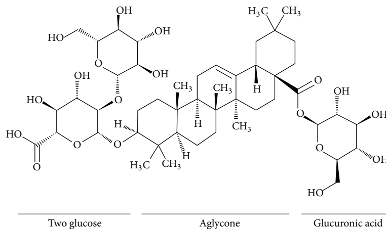
FIGURE 1: Chemical structure of ginsenoside Ro. Ginsenoside Ro (G-Ro), an oleanane-type saponin, is contained in Panax ginseng Meyer [19, 20] and is composed of oleanolic acid as aglycone and two glucose and one glucuronic acid as sugar component [19].
