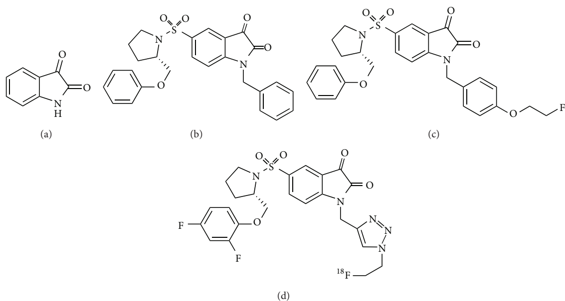
FIGURE 5: Structures of (a) Isatin, (b) (S)-1-benzyl-5-[1-[2-(phoxymethyl)pyrrolidinyl]sulfonyl]isatin, (c) WC-II-89, and (d) [ 18 F]ICMT-11.
