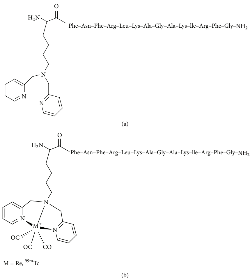
FIGURE 2: Structures of (a) SAAC-PSBP-6 and (b) SAAC(Re)-PSBP-6 and SAAC( 99m Tc)-PSBP-6.
