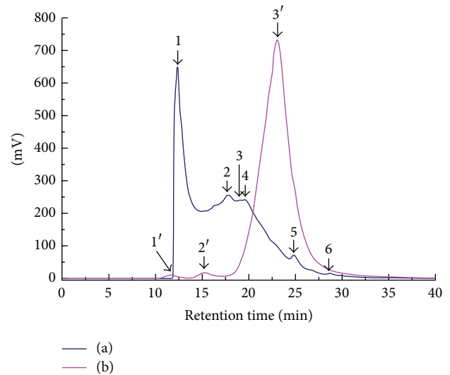
FIGURE 1: HPLC profiles of collagen peptide of deer sinew. Note: (a) collagen of deer sinew was extracted in boiling water. (b) Collagen peptide was treated with trypsin (1 : 1000, w/w) at 37°C for 3 h after boiling water.
