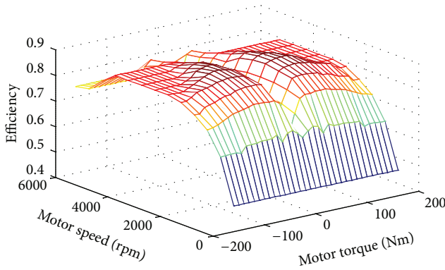
FIGURE 2: Efficiency characteristics of the electric motor.
