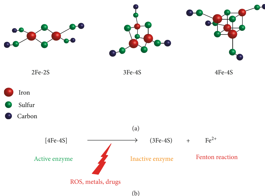
FIGURE 1: Most common iron-sulfur structures. (a) Most common Fe-S clusters associated with proteins contain 2, 3, or 4 iron atoms. Oxidation states of the cluster are variable and can be [2Fe-2S]^+ or [2Fe-2S]^{2+} , [3Fe-4S]^+ , [3Fe-4S]^0 , [3Fe-4S]^- or [3Fe-4S]^{2-} , and [4Fe-4S]^{3+} , [4Fe-4S]^{2+} , [4Fe-4S]^+ , or [4Fe-4S]^0 . [3Fe-4S] clusters are most often considered as deriving from [4Fe-4S] clusters that have been oxidized by various cellular oxidants. Iron atoms are shown in red, sulfur atoms are shown in green, and carbon from cysteine residues are shown in dark blue. Coordination by histidine is not shown. (b) Conversion of [4Fe-4S] into [3Fe-4S] clusters is responsible for Fe^{2+} release and for enzyme inactivation. Fe^{2+} release might lead to Fenton reactions in the presence of hydrogen peroxide.
