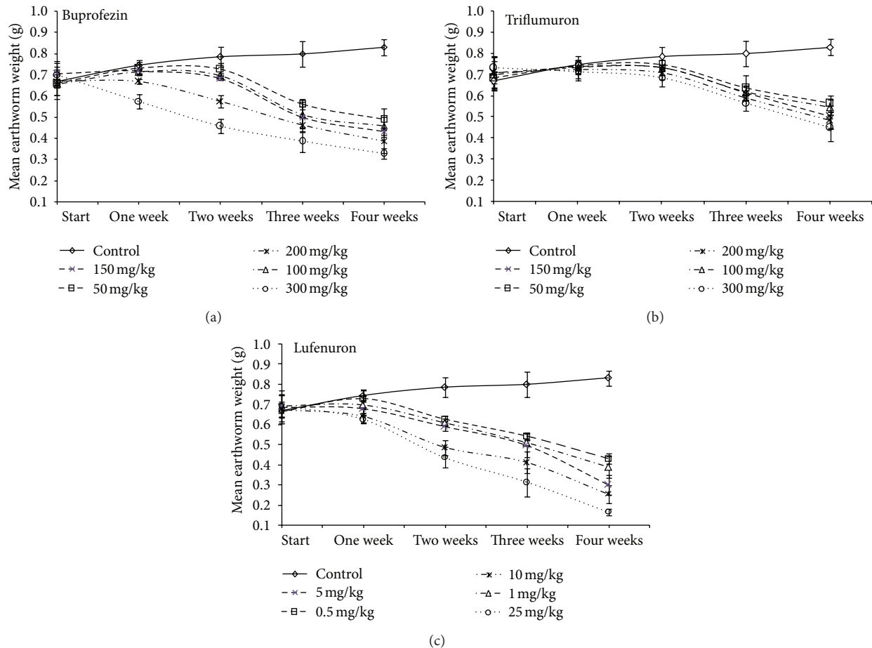
FIGURE 1: Mean weight \pm SD of earthworms A. caliginosa in artificial soil treated with buprofezin, triflumuron, and lufenuron at different application rates in the laboratory. Growth weight measured when experiment started and 1, 2, 3, and 4 weeks after treatment.
