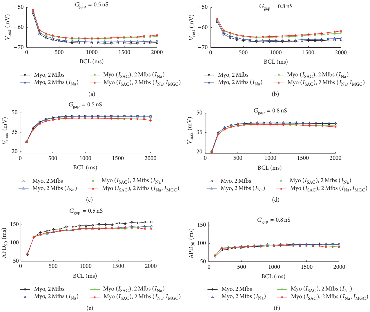
FIGURE 6: Effects of I_{SAC} , I_{Na\_Mfb} , and I_{MGC\_Mfb} on AP characteristics as a function of BCL in Mfb-M coupling with I_{Na\_Mfb} (blue line with hollow triangle), with I_{SAC} and I_{Na\_Mfb} (green line with hollow rectangle), and with I_{SAC} , I_{Na\_Mfb} , and I_{MGC} (red line with asterisk) as compared to control (black line with hollow circle), by coupling two Mfbs to an atrial myocyte with G_{gap} of 0.5 and 8 nS. (a, b) V_{rest} , (c, d) V_{max} , and (e, f) APD_{90} .
