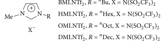
FIGURE 1: Schematic representation of ILs structures.
