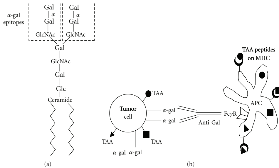
FIGURE 1: (a) Ceramide decahexoside as a representative \alpha -gal glycolipid. This glycolipid has 10 carbohydrate branched chain. The \alpha -gal epitope ( \text{Gal}\alpha 1\text{-}3\text{Gal}\beta 1\text{-}4\text{GlcNAc-R} ) marked by the broken line rectangles caps both carbohydrate branches. The terminal \alpha -galactosyl (Gal) unit is linked \alpha 1,3 to the penultimate Gal of the carbohydrate chain by the glycosylation enzyme \alpha 1,3 galactosyltransferase ( \alpha 1,3\text{GT} ). The lipid portion of \alpha -gal glycolipids (ceramide) anchors the carbohydrate portion in the cell membrane via the two fatty acid tails. (b) Anti-Gal-mediated targeting of tumor cells to APC in lesions injected with \alpha -gal glycolipids. Intratumoral injection of \alpha -gal glycolipids results in insertion of these glycolipids in tumor cell membranes. Anti-Gal IgG binds in situ to \alpha -gal epitopes on the inserted glycolipids. Subsequent interaction between the Fc portion of the bound anti-Gal and Fc \gamma R on the APC (illustrated as a dendritic cell) induces uptake of intact or lysed tumor cells by APC, resulting in effective internalization of the tumor-associated antigens (TAA). Internalized TAA are processed and various immunogenic TAA peptides ( \bullet , \blacksquare , \blacktriangle ) are presented by the APC in association with class I and class II MHC molecules. These immunogenic peptides can activate tumor specific cytotoxic and helper T cells and elicit a protective antitumor immune response.
