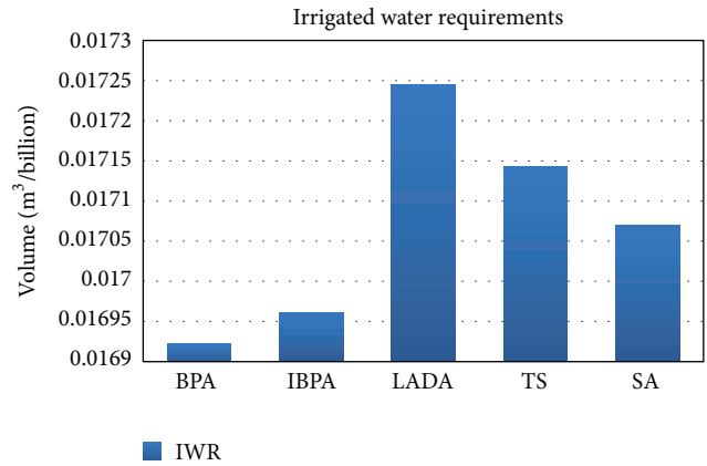
FIGURE 5: Irrigated Water Requirements (IWR) of the best heuristic solutions.
