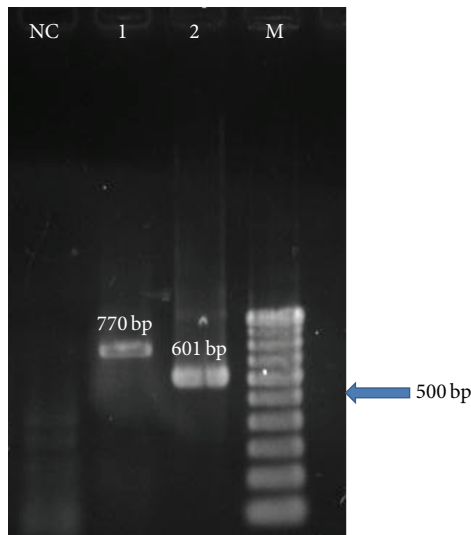
FIGURE 1: Nested RT-PCR assay used to detect FeLV U3LTR-gag sequence from naturally infected cats in Malaysia. The outer PCR reaction was performed using primer pair U3-F(1) and G-R(1) and amplified 770 bp (lane 1) whilst inner PCR reaction was performed using primer pair U3-F(2) and G-R(2) and amplified 601 bp (lane 2). Lane NC: negative control, lane M: 100 bp DNA marker (iDNA, Malaysia).
