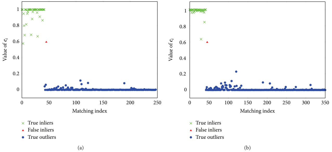
FIGURE 2: Distribution of C which represents the contribution of each matching to the optimization problem. Also, it is an indicator of outliers as we classify \mathbf{m}_i as outlier if c_i < 0.5 . Without loss of generality, inliers are put in the first 42 indexes. (a) Test with 206 outliers in which 1 false inlier appeared. (b) Test with 309 outliers in which 1 false inlier appeared.
