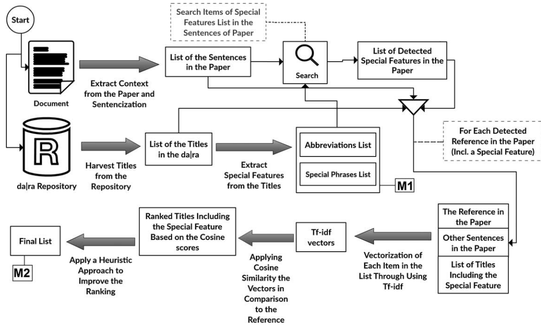
Fig. 3. An overview of the approach.
