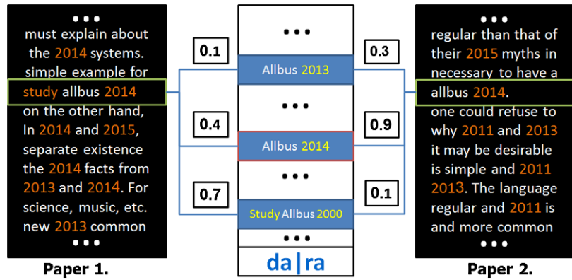
Fig. 2. A toy example of cosine similarity, where tf-idf is computed over phrases in two articles.
