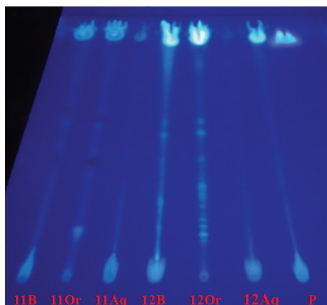
FIGURE 2: TLC of CEDp11 and CEC12 samples and their respective fractions, visualized at UV365 nm. Mobile phase: toluene : ethyl acetate (75 : 25 v/v). 11B: crude extract; 11Or: organic fraction; 11Aq: aqueous fraction; 12B: crude extract; 12Or: organic fraction; 12Aq: aqueous fraction; P: quercetin standard.
