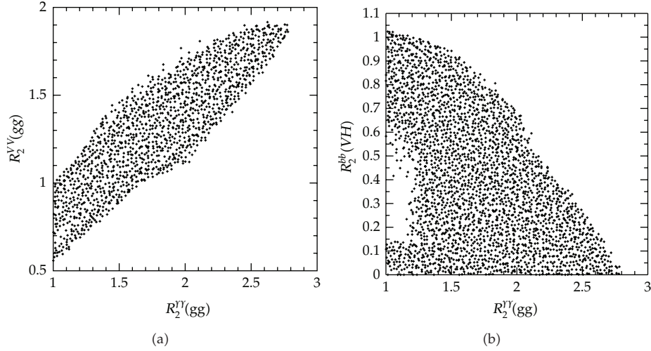
Figure 2: (a) R_2^{VV}(gg) as function of R_2^{\gamma\gamma}(gg) . (b) R_2^{bb}(VH) (associate production W/Z+H_2 with H_2 \rightarrow b\bar{b} ) as a function of R_2^{\gamma\gamma}(gg) .
