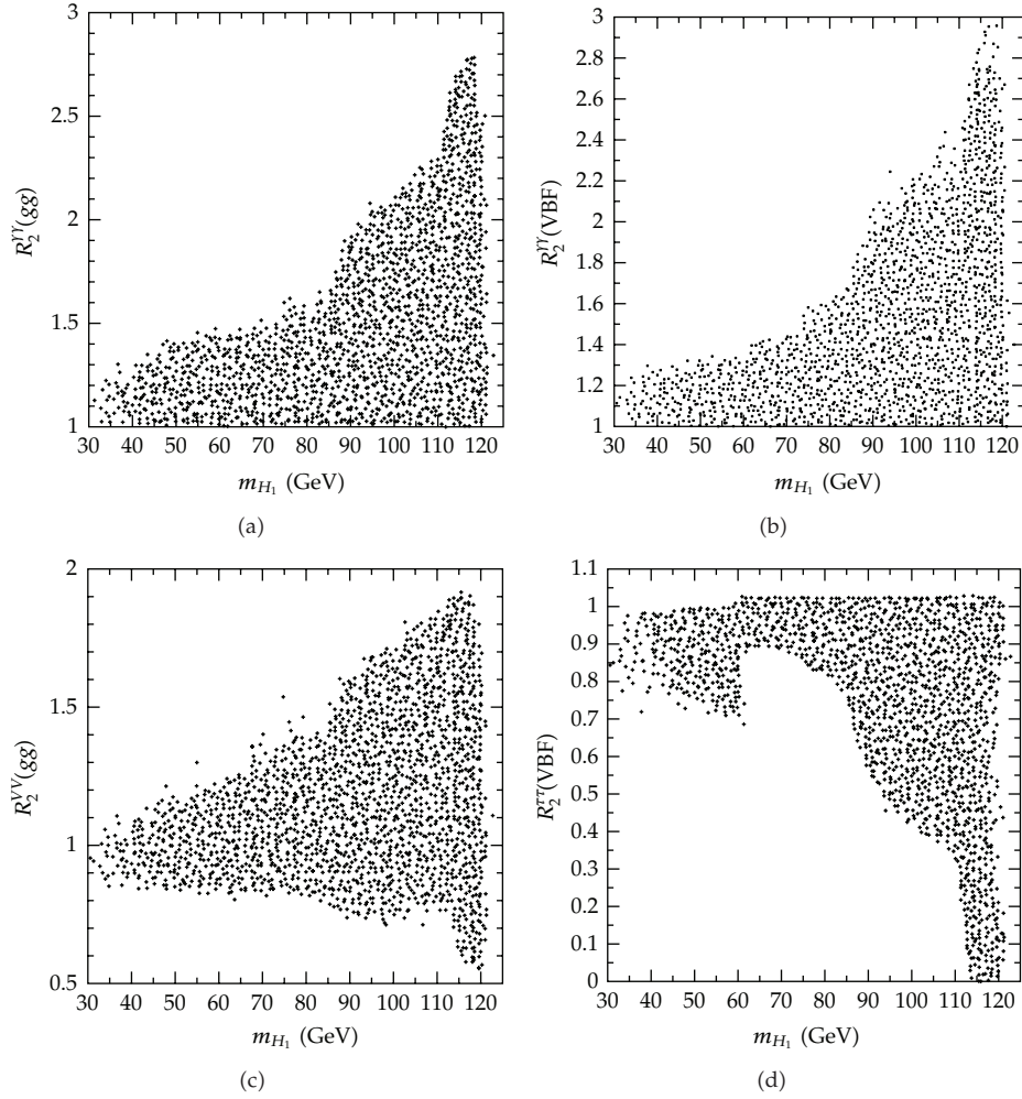
Figure 1: Reduced signal cross sections R_2 for H_2 with a mass in the 124–127 GeV range, as a function of M_{H_1} for a representative sample of viable points in parameter space. (a) R_2^{\gamma\gamma}(gg) (diphoton channel, H_2 production via gluon fusion), (b) R_2^{\gamma\gamma}(VBF) (diphoton channel, H_2 production via VBF), (c) R_2^{VV}(gg) ( ZZ , WW channels, H_2 production via gluon fusion), and (d) R_2^{\tau\tau}(VBF) ( \tau\tau channel, H_2 production via VBF).
