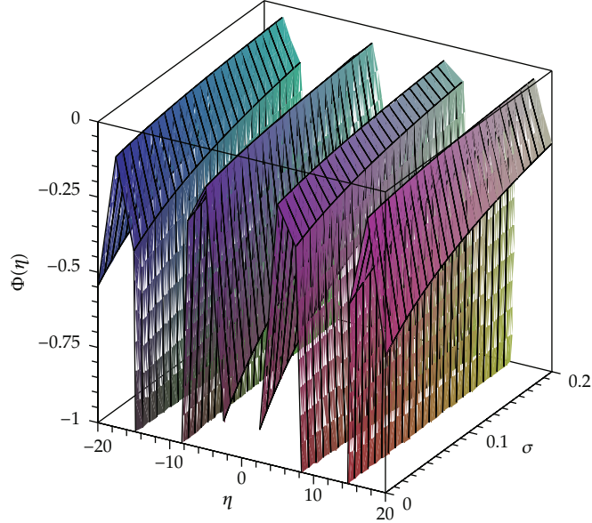
Figure 5: Weierstrass elliptic doubly periodic type solution (4.13) for v = 0.04 , \gamma_0 = 0.01 , c_0 = -1 , c_1 = 1 , and c_3 = 0.1 .
