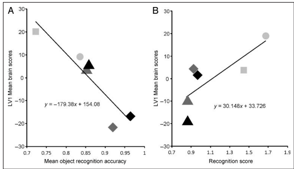
Figure 5. Relationship between brain scores and recognition performance. (A) Regression between brain scores in LV1 and object recognition accuracy. Increases in activation in regions associated with LV1 (see Figure 3) are accompanied by decreases in overall recognition accuracy. (B) Regression between brain scores in LV2 and the recognition scores. Recognition scores reflect the summed accuracy for left and right objects in the bilateral condition. As can be seen, all low-load conditions fall above the regression line, whereas all high-load conditions fall below it. Thus, increases in activation in regions
