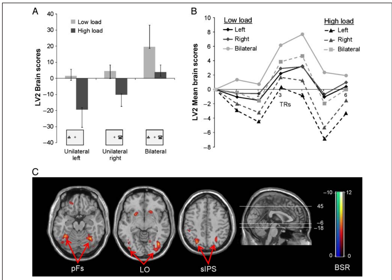
Figure 4. Brain scores and peak clusters for LV2. (A) Mean brain scores as a function of VWM load and object presentation condition. Brain scores reflect the activation summed across the entire brain and averaged across participants. Higher brain scores are observed in the low-load condition relative to the high-load condition, and scores are greater when two objects are presented relative to only a single object. Error bars denote 95% confidence intervals. (B) Mean brain scores observed in LV2 as a function of time (TRs). Overall, the brain scores peak later in the trial relative to the scores in LV1 (see Figure 3). (C) Peak cluster activations observed in LV2 extracted from TR4. BSRs are displayed. The z axis of the MNI coordinates of each slice is indicated. Regions identified in LV2 largely correspond to object-sensitive LOC, containing the posterior fusiform sulcus (pFs) and lateral occipital (LO) regions. In addition, a similar pattern of activation was also observed in sIPS.
