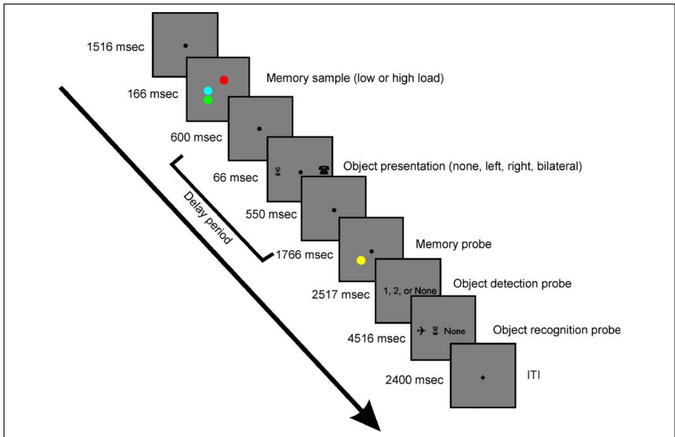
Figure 1. Schematic of experimental trials. The trial begins with a fixation period, immediately followed by the memory sample of the change detection task. The memory load was manipulated by presenting either one (low load) or three (high load) memory items. Participants are told to remember as many of the colored items over the 1216-msec delay period as possible. Half-way through the delay period, participants were presented with one object (unilaterally on the left or right), two objects (bilaterally on the left and right), or no objects. Following the remaining delay, participants were given a memory probe, in which they indicated whether the probe item was a different color from the original memory sample (50% of trials). Immediately following the memory probe, object detection (Experiment 1) and object recognition (Experiments 1 and 2) probes were given.
