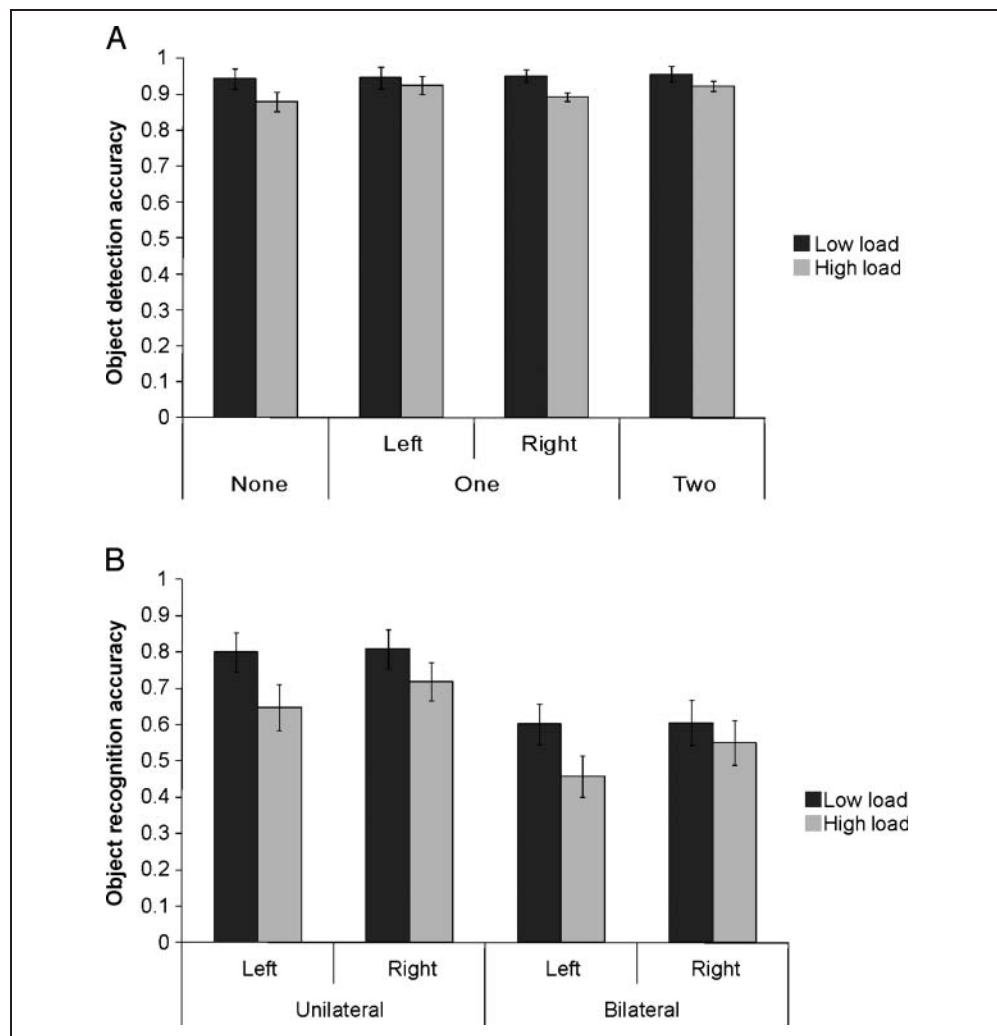
Figure 2. Experiment 1: Detection and recognition performance. (A) The proportion of correct responses (hits–false alarms) to the object detection probe as a function of memory load and object presentation condition. Object detection performance is largely unaffected by memory load or object condition. (B) The proportion of correctly identified objects in the object detection probe as a function of memory load and object presentation condition. Under a high VWM load, recognition performance is particularly impaired for objects presented in the left visual field. Error bars denote SEMs .
