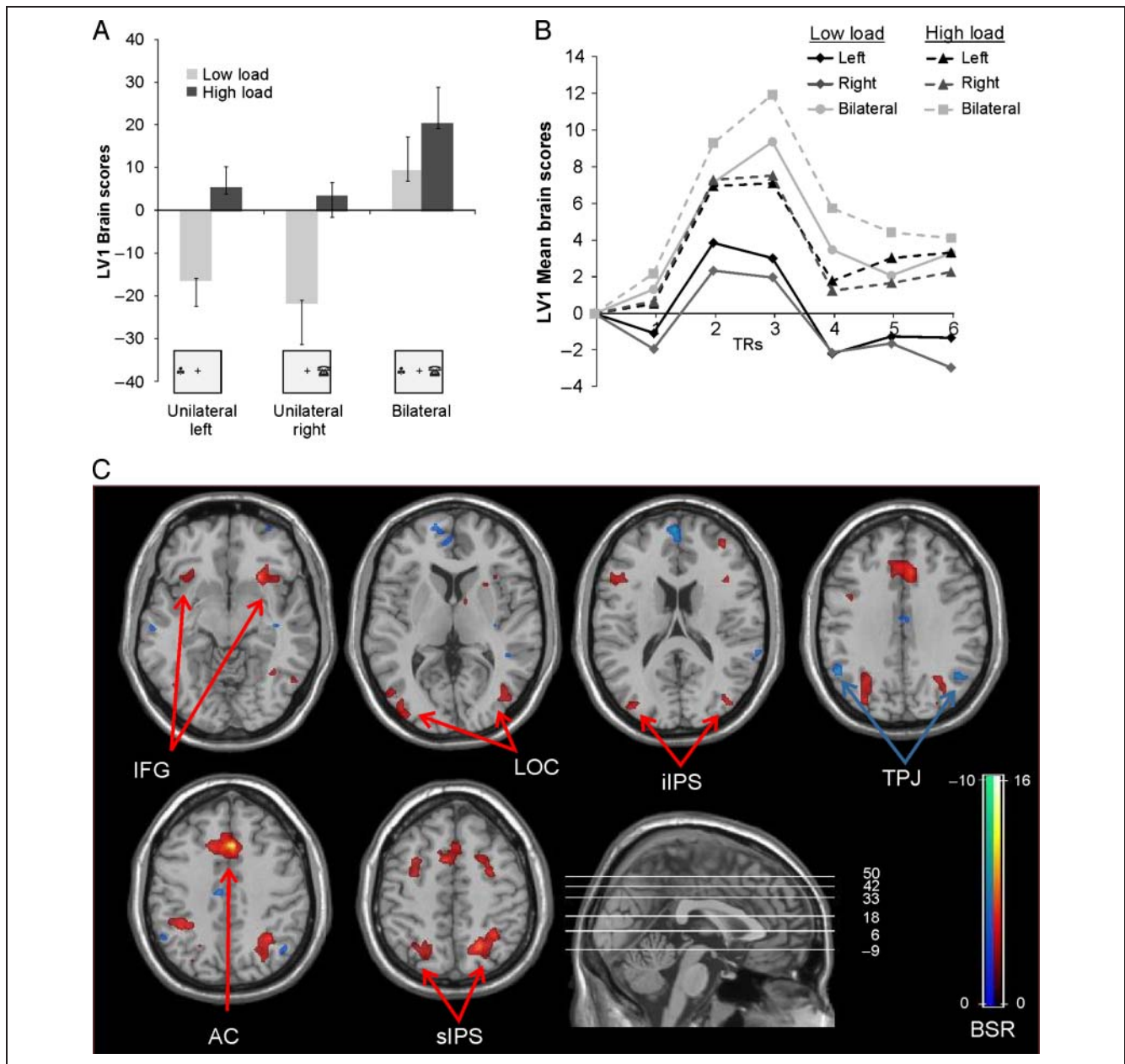
Figure 3. Brain scores and peak clusters for LV1. (A) Mean brain scores as a function of VWM load and object presentation condition. Brain scores reflect the activation summed across the entire brain and averaged across participants. Higher brain scores are observed in the high-load condition relative to the low-load condition, and scores are greater when two objects are presented relative to only a single object. Error bars denote 95% confidence intervals. (B) Mean brain scores observed in LV1 as a function of time (TRs). The diverging effects of VWM load and number of objects can be observed. (C) Peak cluster activations observed in LV1 extracted from TR2. BSRs are displayed. The z axis of the MNI coordinates of each slice is indicated. Regions corresponding to areas previously demonstrated as being sensitive to VWM load are identified.
