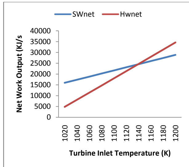
Figure 9: effect of turbine inlet temperature on network output of gas turbine
