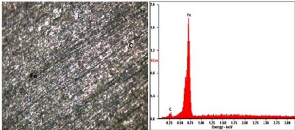
Figure 1:SEM/EDS spectra of as-received mild steel
