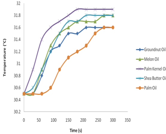
Figure 1. The rate of heat extraction of different bio-quenching oils at 200°C.
