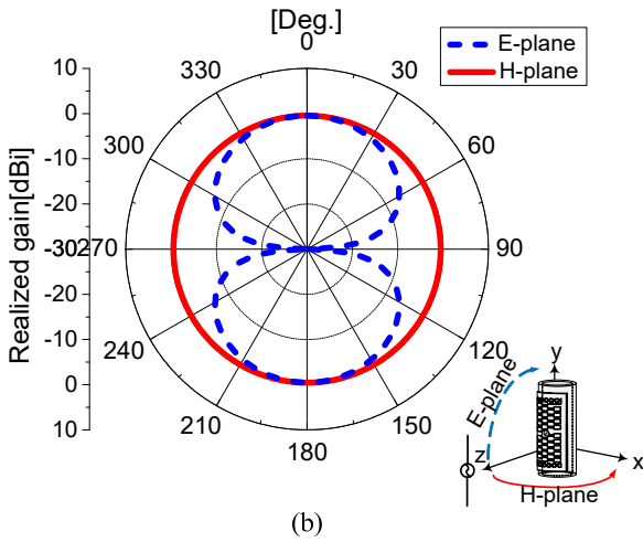
Fig. 5. Return loss and radiation pattern of the proposed antenna (simulation). (a) S_{11} . (b) Radiation pattern.
