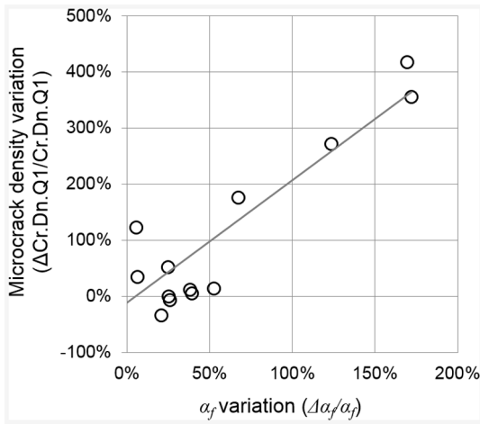
Figure 7. Correlation between the relative variation \Delta\alpha_f/\alpha_f of the nonlinear elastic parameter ( \alpha_f represents the difference between the initial value and the value measured after the last damage step) and the relative variation of short microcracks density \Delta\text{Cr.Dn.Q1}/\text{Cr.Dn.Q1} between VOI1 and VOI2. One specimen (#6; \Delta\text{Cr.Dn.Q1}/\text{Cr.Dn.Q1}=0.36 ; \Delta\alpha_f/\alpha_f=2.48 ) exhibiting the strongest \alpha_f variation is not represented doi:10.1371/journal.pone.0083599.g007
