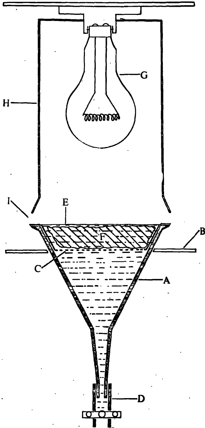
Fig. 13. The wet funnel extractor.
