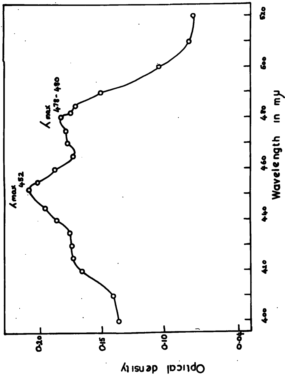
Figure 28 Absorption spectrum of orange pigment extracted from cultures grown in darkness.
